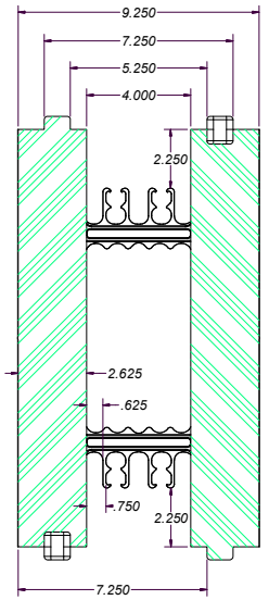
SECTION B-B SCALE 1/2
